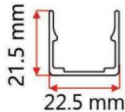
铝槽尺寸 Aluminum Profile size(mm)
